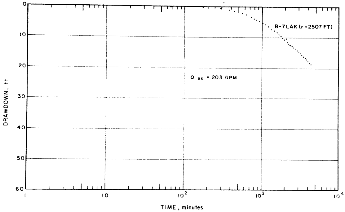
Figure (2): Semilogarithmic Graph of Drawdown for B-7 Observation Well Group, Lakota Aquifer Test
