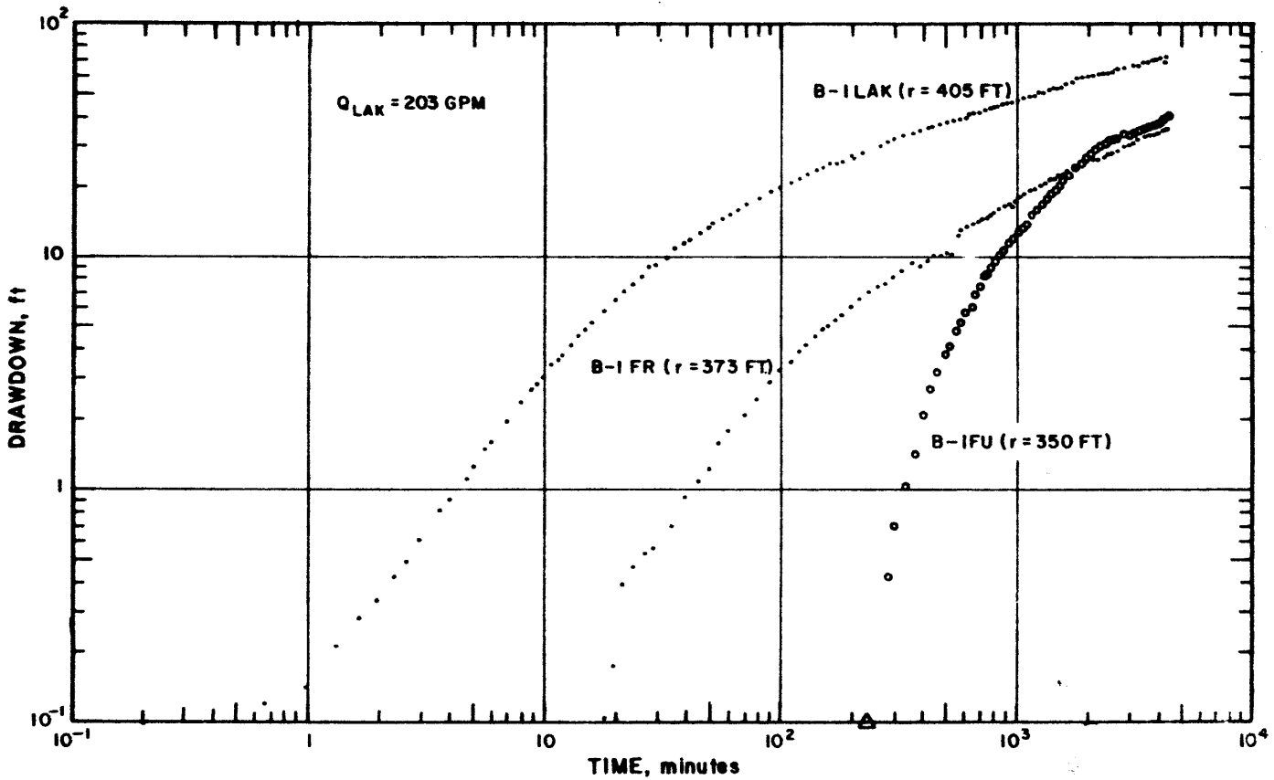
Figure 14 : Logarithmic Graphs of Drawdown for B- I Observation Well Group, Lakota Aquifer Test
