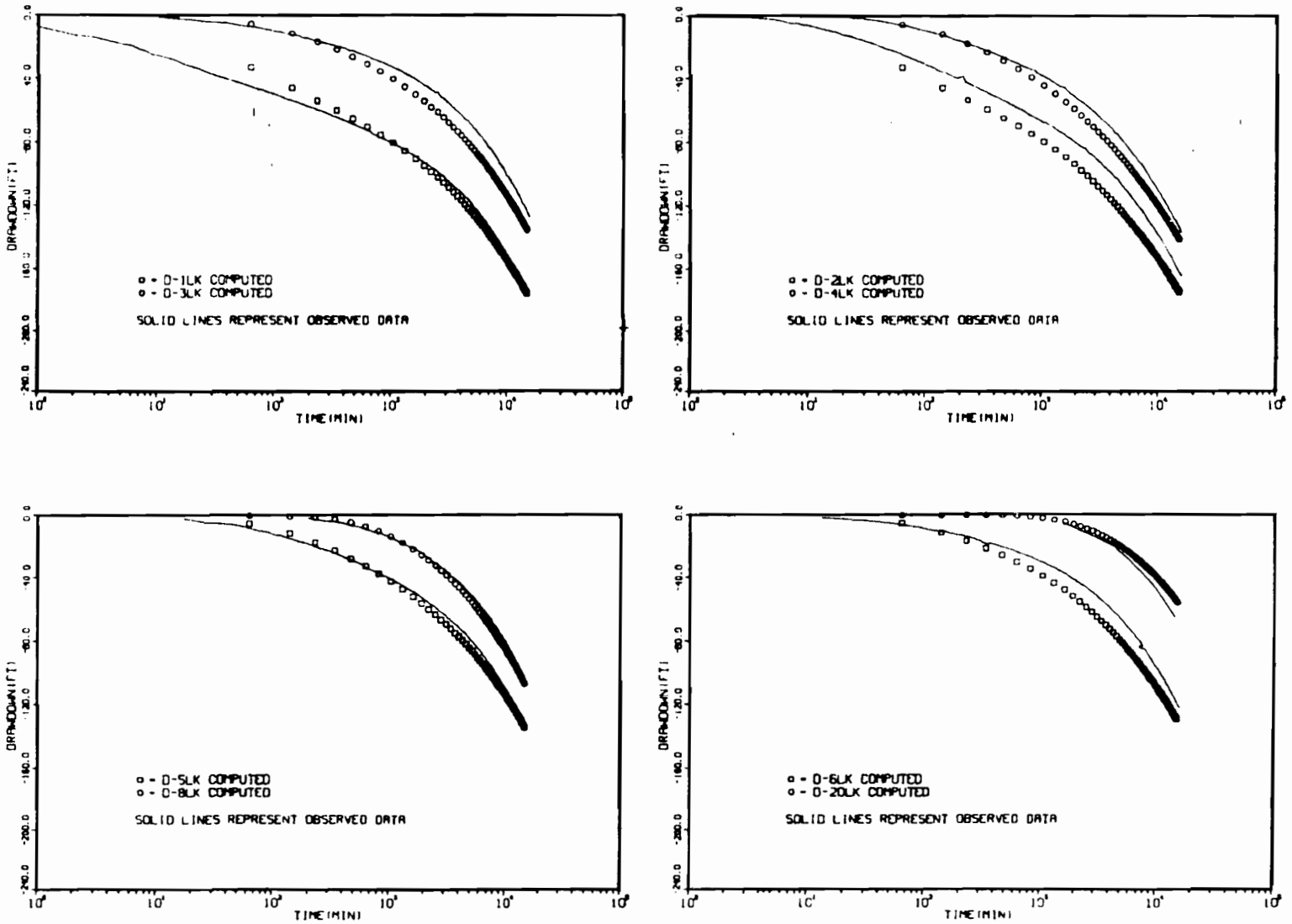
Figure 7. Comparison of Observed and Computed Drawdown, Case II
