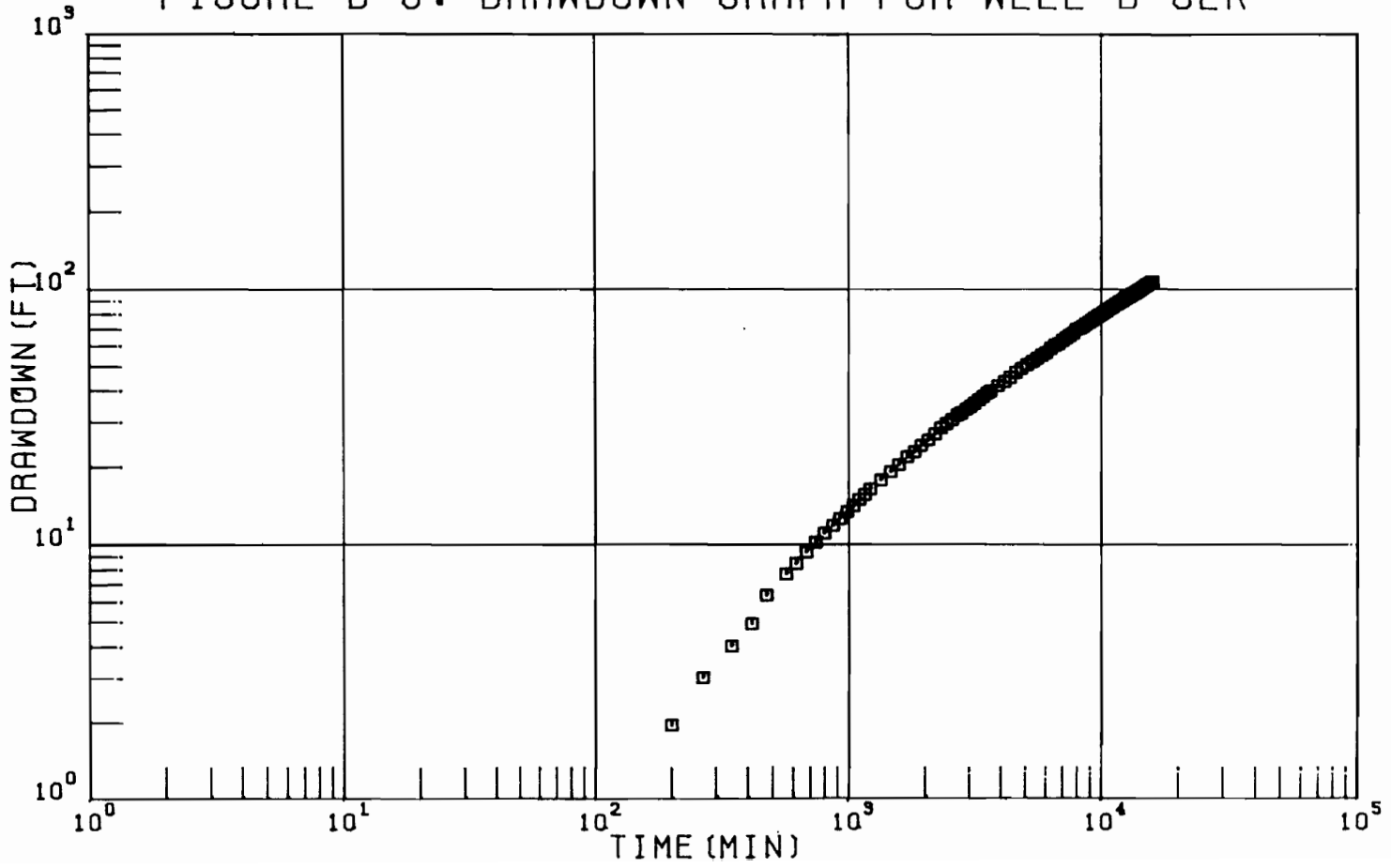
FIGURE B-8: DRAWDOWN GRAPH FOR WELL D-8LK
