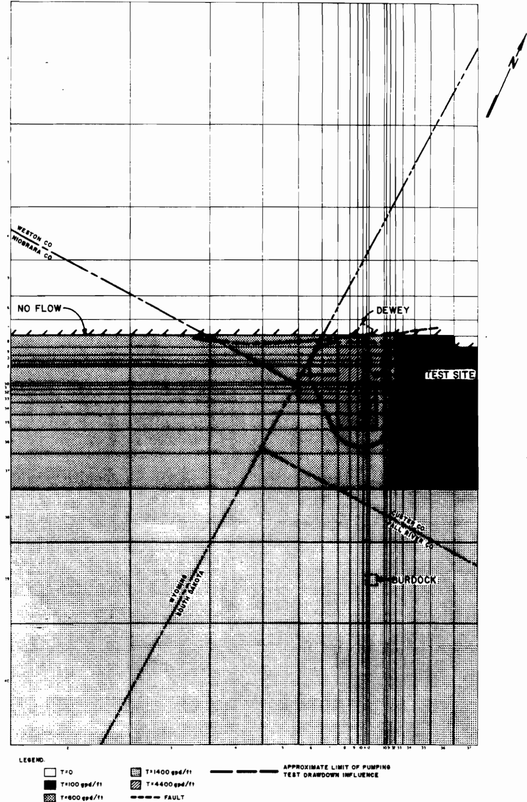
Figure 6: Transmissivity Distribution, Case II
