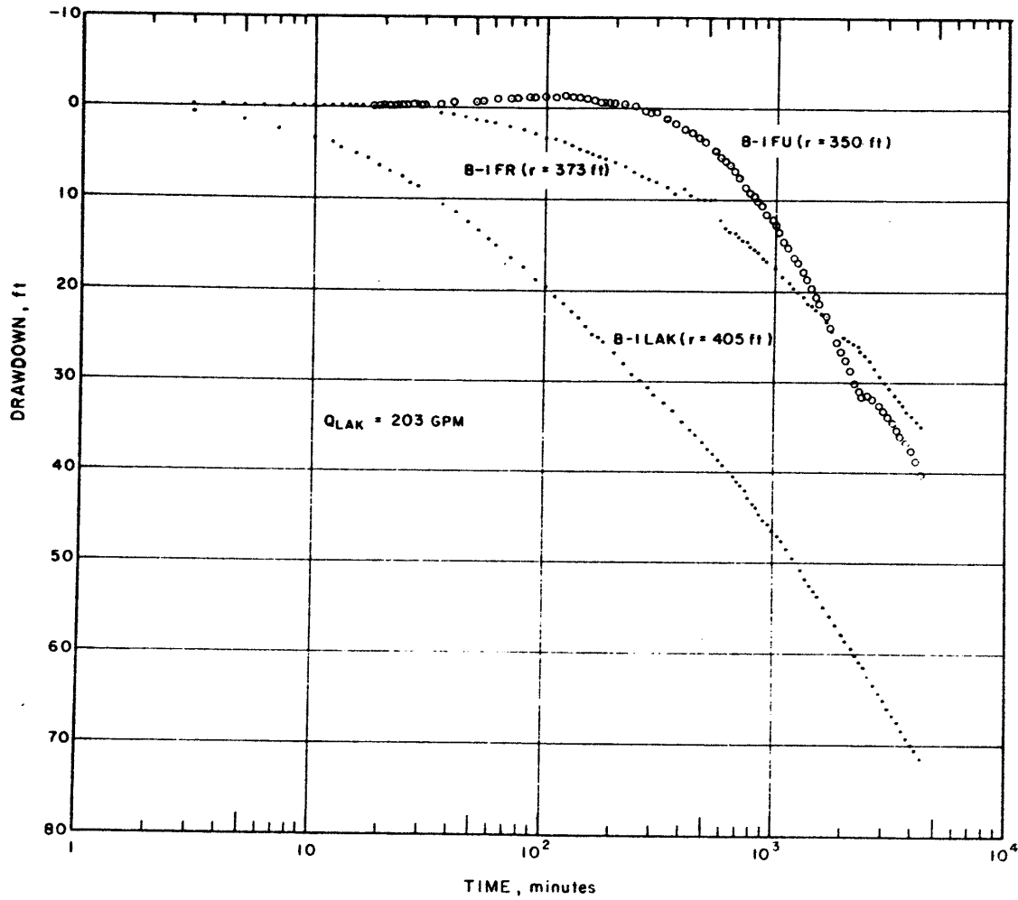
Figure 9: Semilogarithmic Graphs of Drawdown for B-1 Observation Well Group, Lakota Aquifer Test
