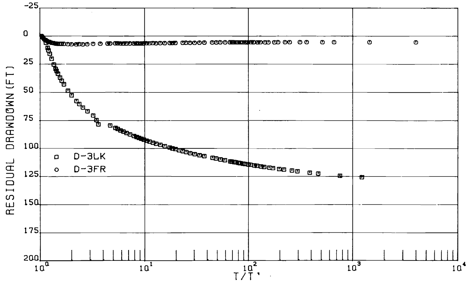
FIGURE C-4: RECOVERY GRAPH FOR D-3 WELL GROUP
