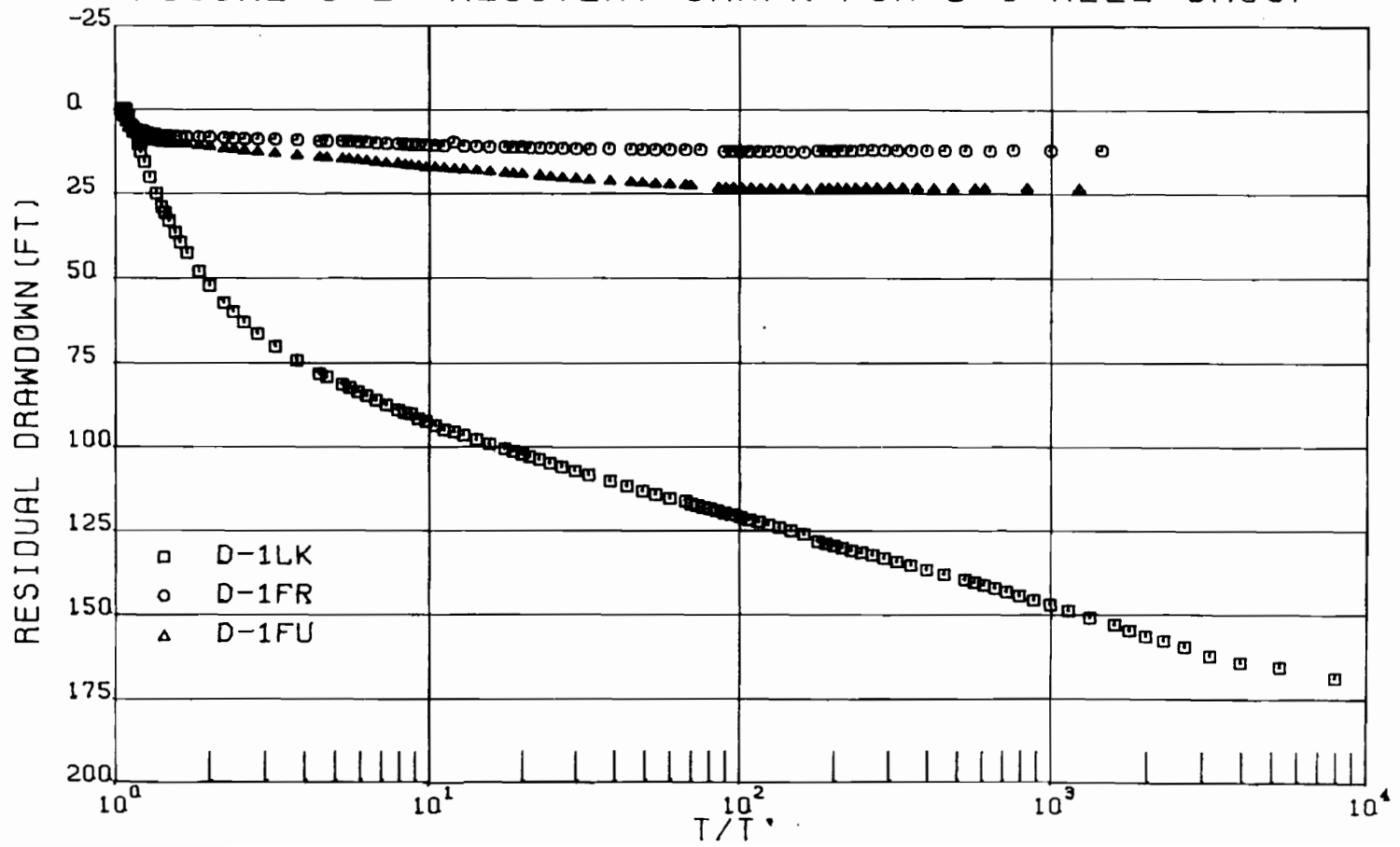
FIGURE C-2: RECOVERY GRAPH FOR D-1 WELL GROUP
