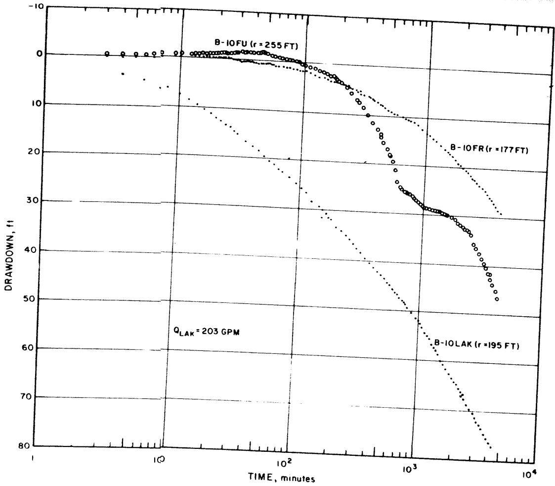
Figure 8 : Semilogarithmic Graphs of Drawdown for B-10 Observation Well Group, Lakota Aquifer Test
