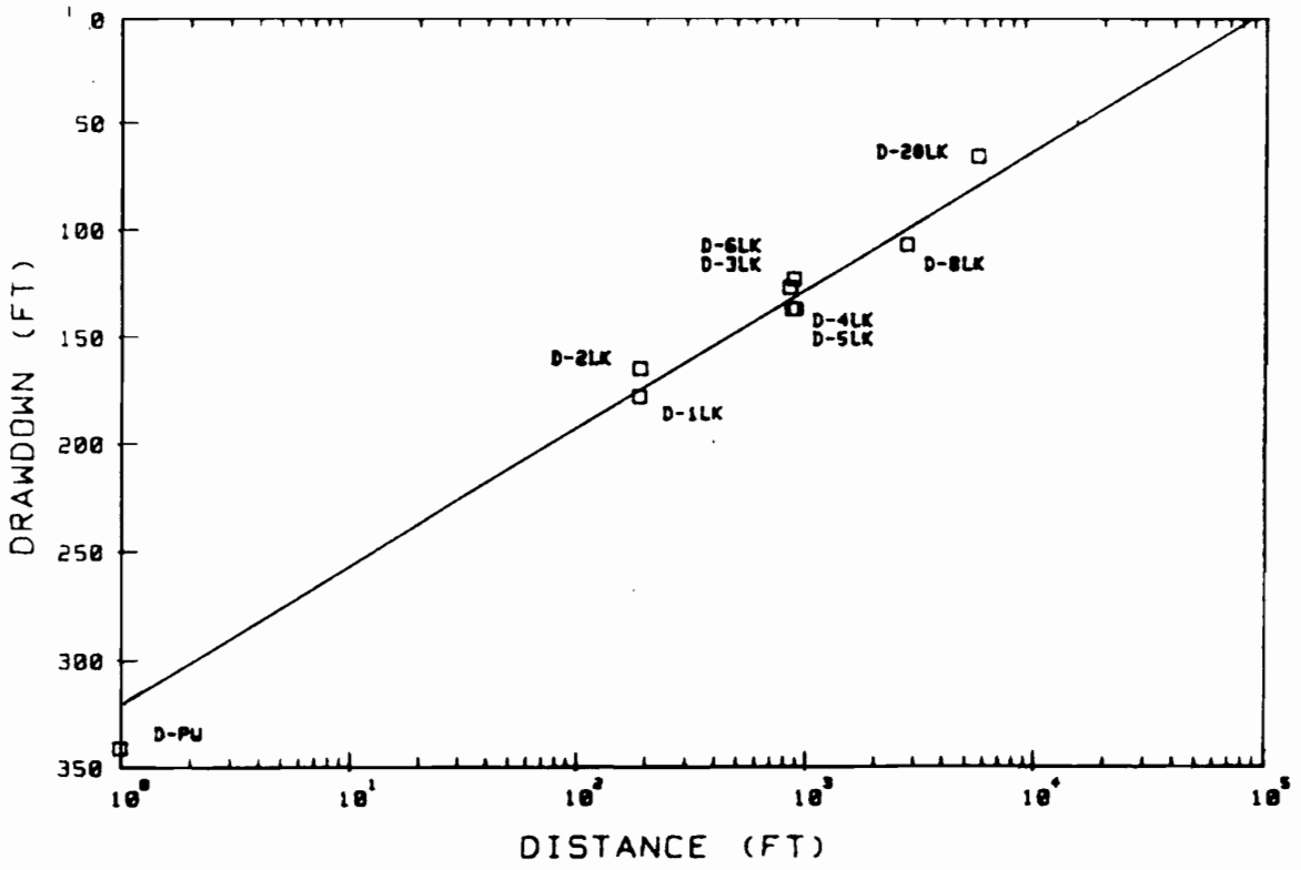
FIGURE 3. DISTANCE-DRAWDOWN GRAPH
